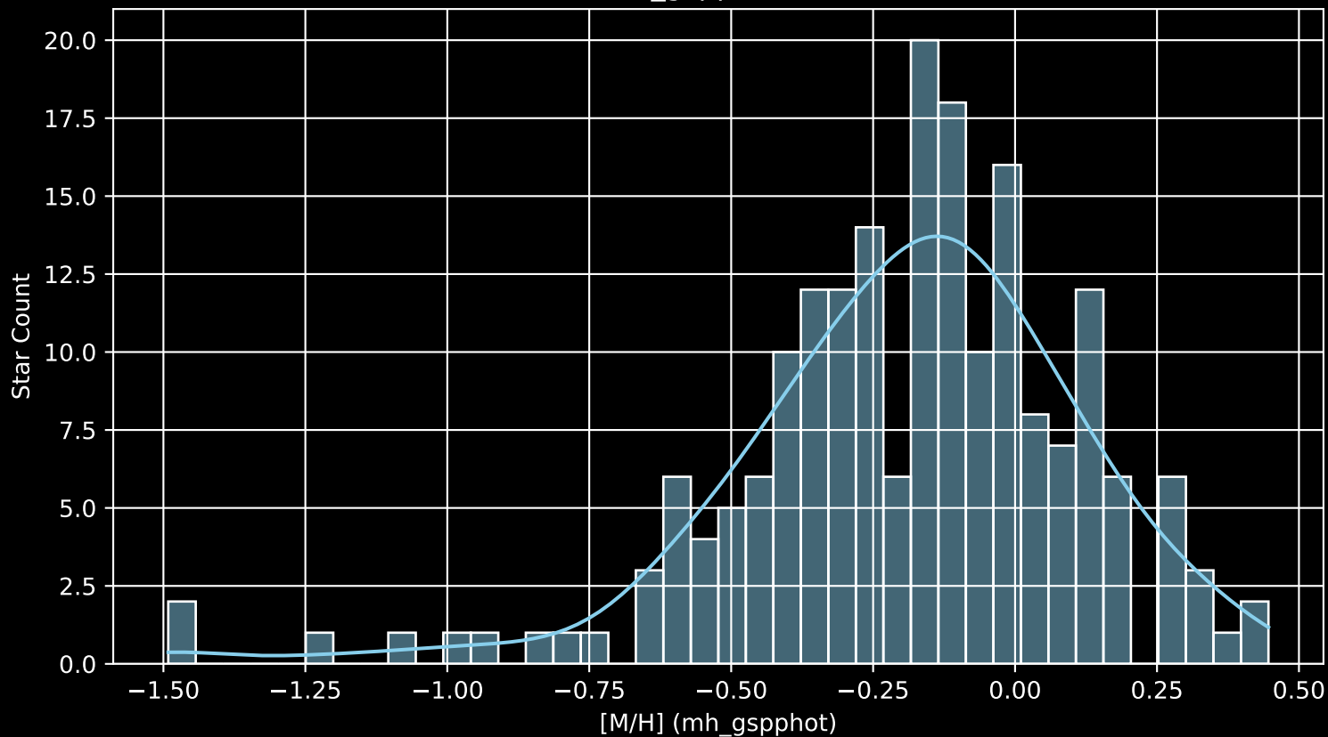
APOGEE DR17 Field: [196+25_MGA [M/H] (mh_gspphot) (n= 196)
