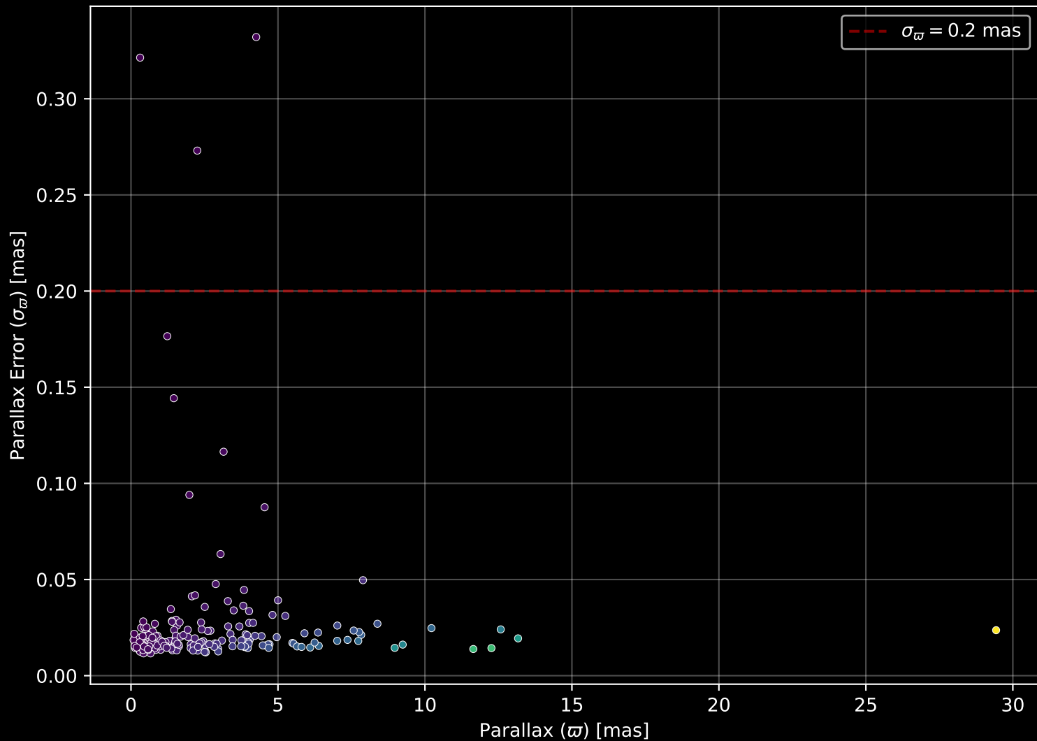
APOGEE DR17 Field: [196+25_MGA] Parallax Quality (n= 199)
