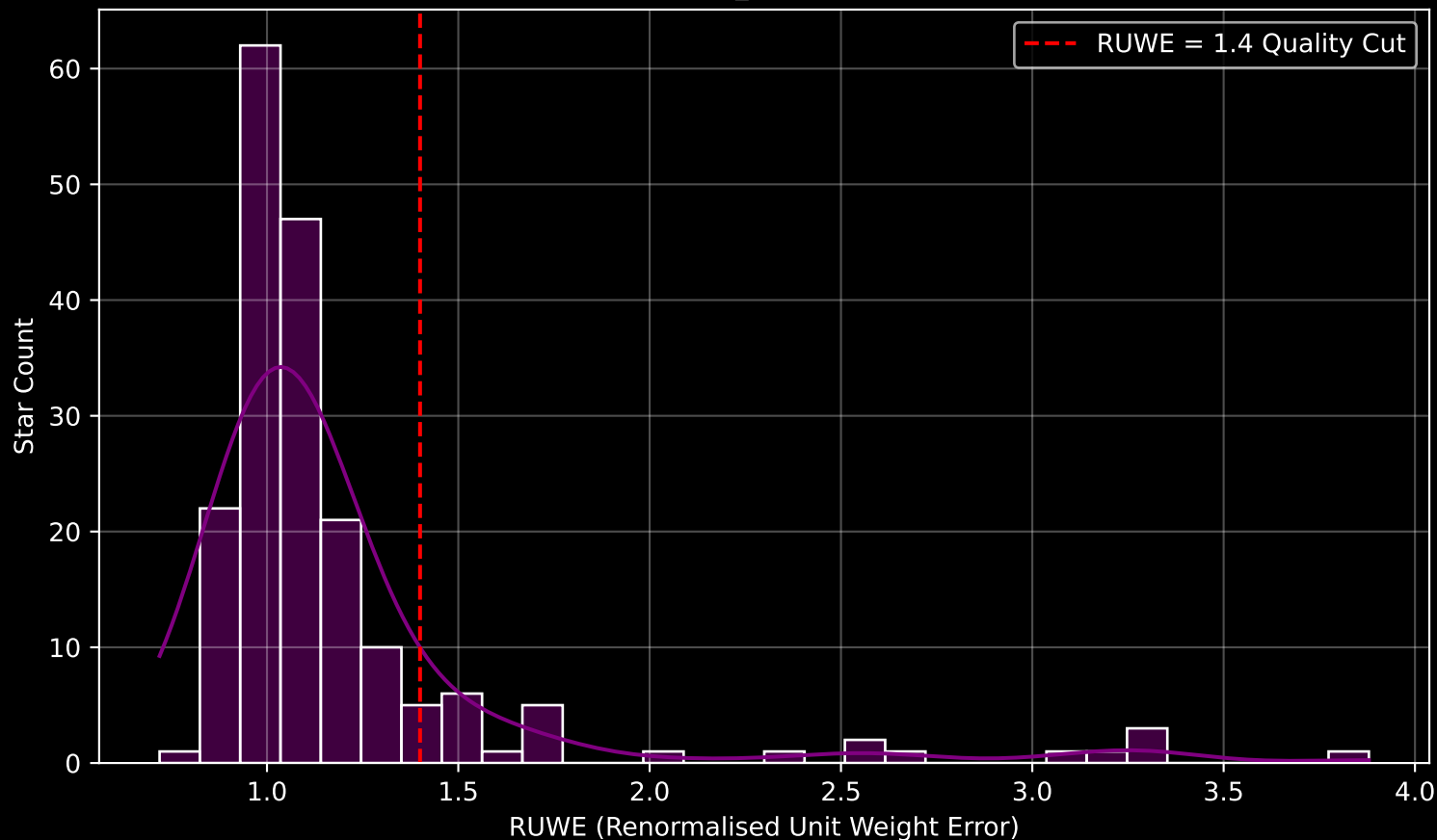
GAPOGEE DR17 Field [196+25_MGA] RUWE Distribution (n= 191)
