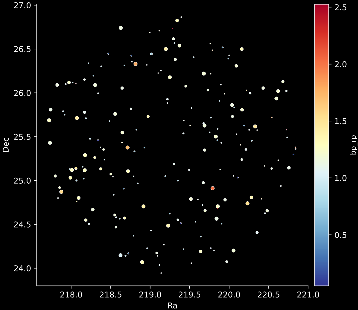
APOGEE DR17 Field: [196+25_MGA] Stars: 199
