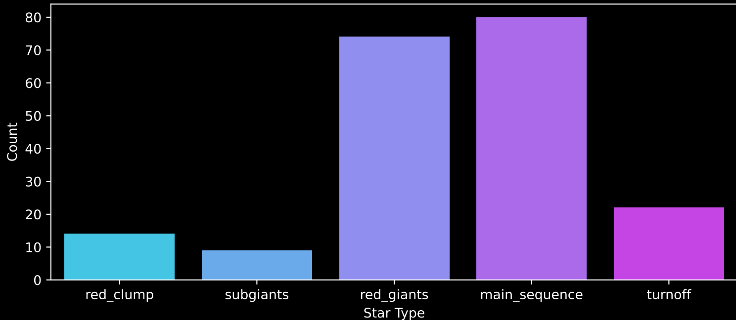
APOGEE DR17 Field: [196+25_MGA] Count plot of Star Type
