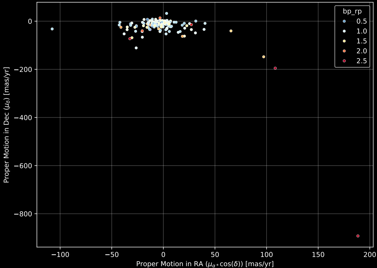
APOGEE DR17 Field: [196+25_MGA] Proper Motion Diagram (n= 199)
