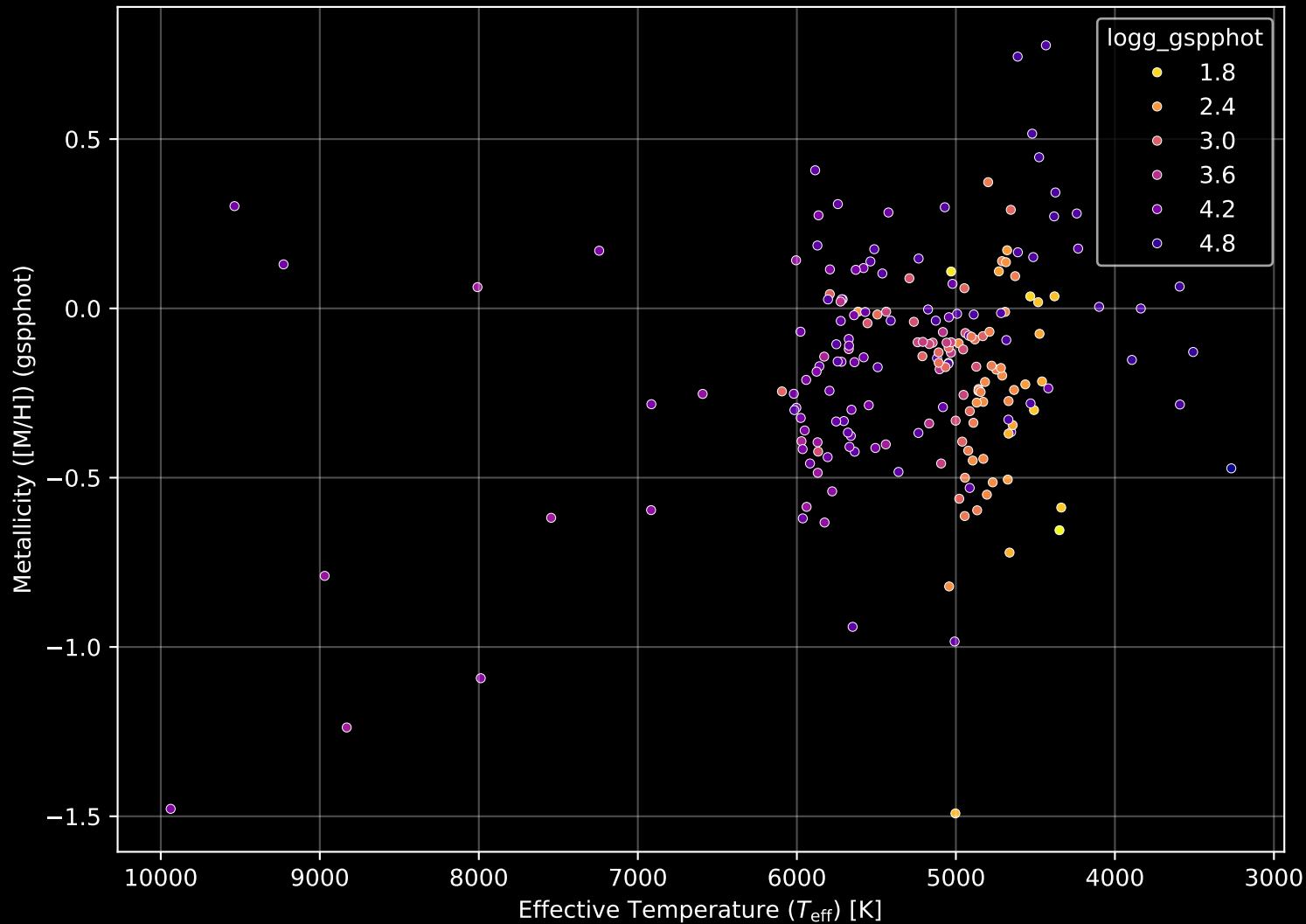
APOGEE DR17 Field: [196+25_MGA] Stellar Population Parameters (n= 199)
